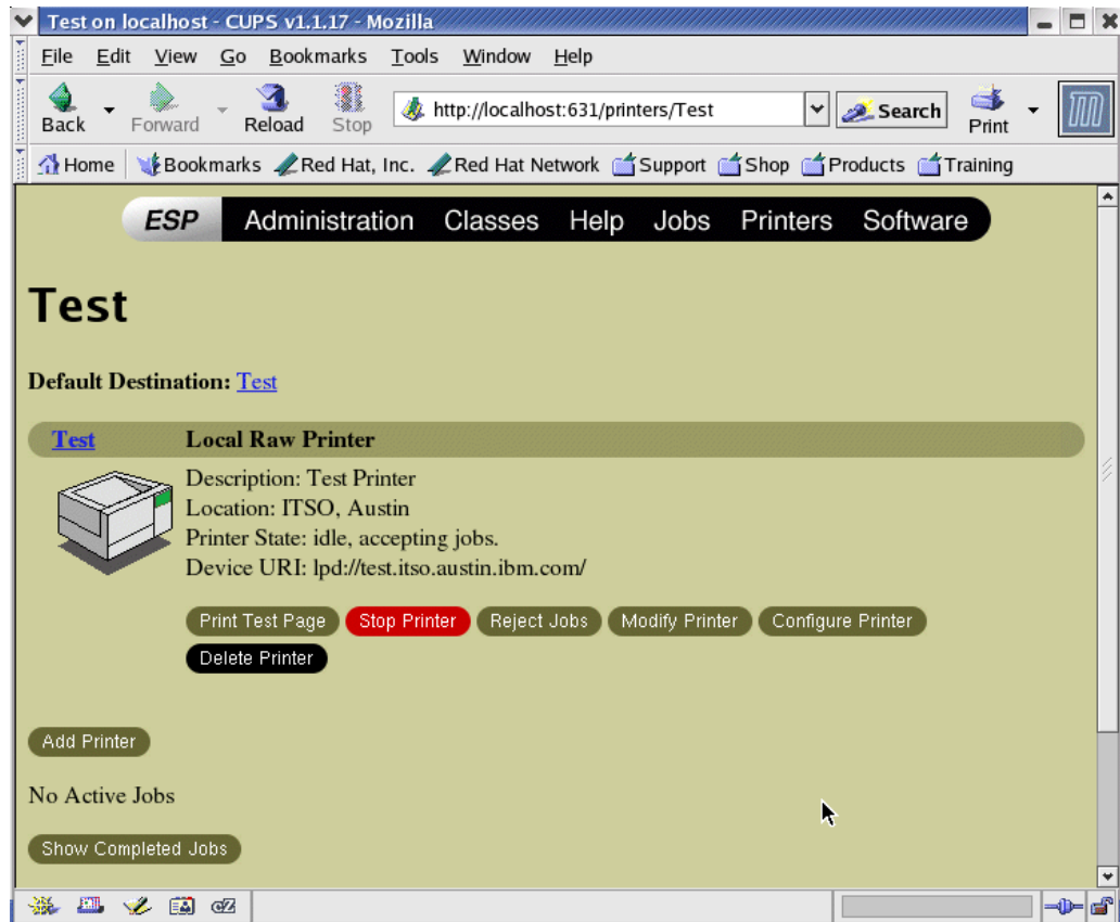
Figure 3-9 CUPS printer status page
