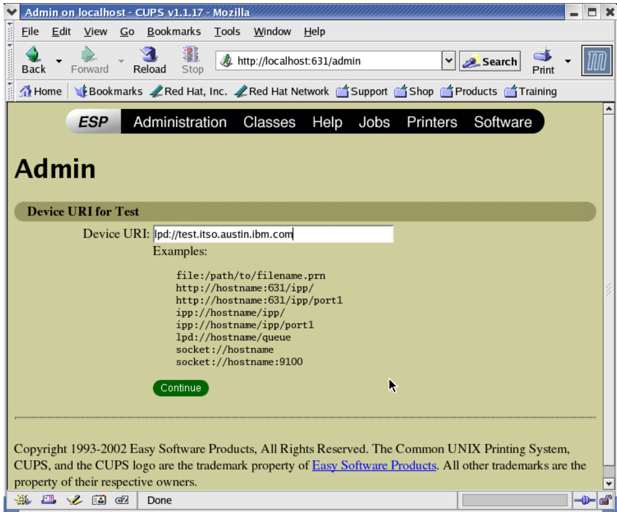
Figure 3-5 URI to printer/print queue
